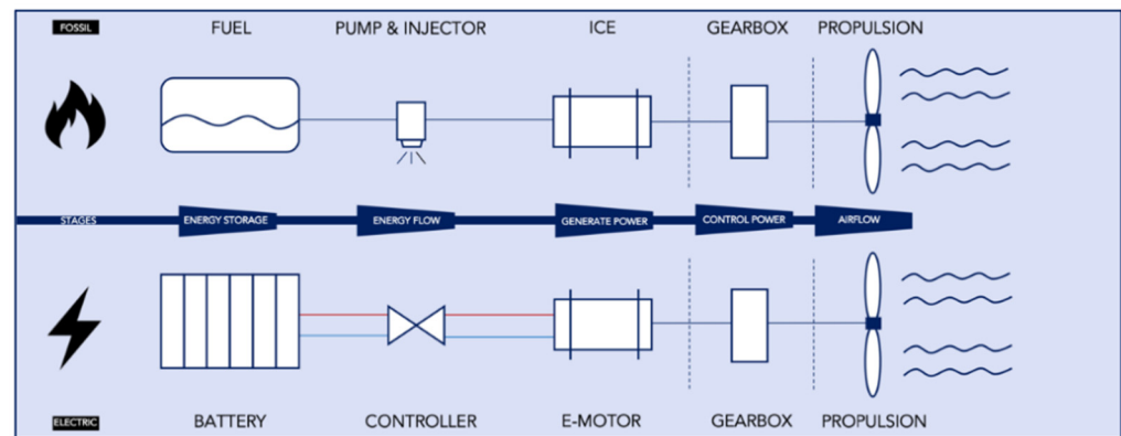
Figure 1. Powertrain in an electric and a conventional small aircraft (adapted from [8]).
