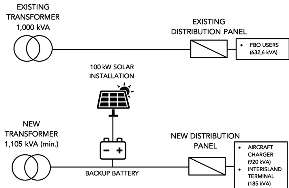
Figure 12. Second concept drawing of a new electric infrastructure to install one charging station.
