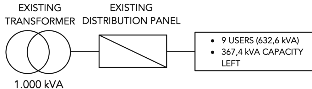
Figure 10. Simple drawing of the current electrical infrastructure on the south side of AUA.
