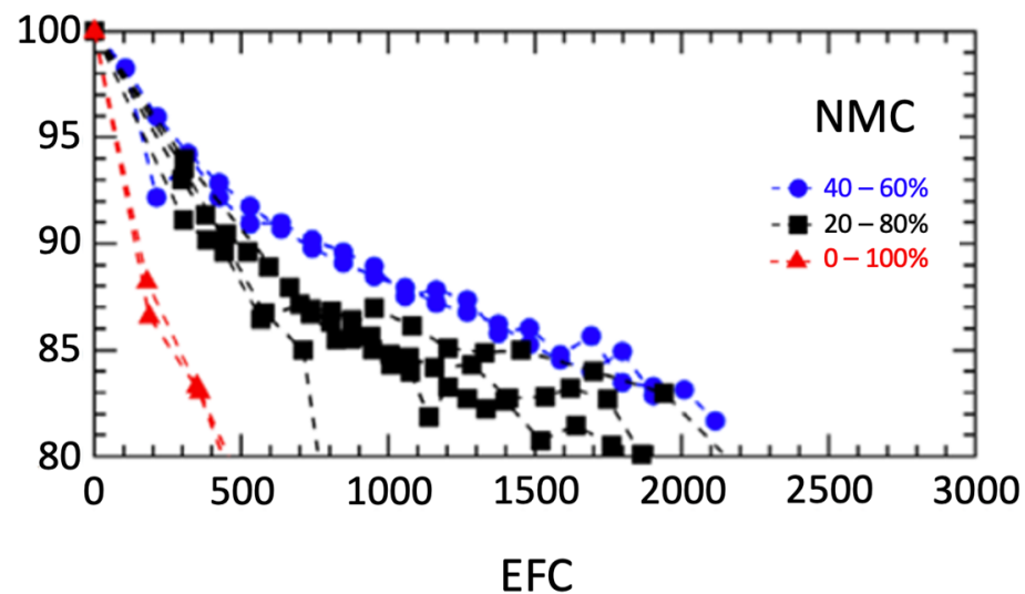
Figure 7. Degradation of NMC Li-ion batteries under different SoC ranges [37].
