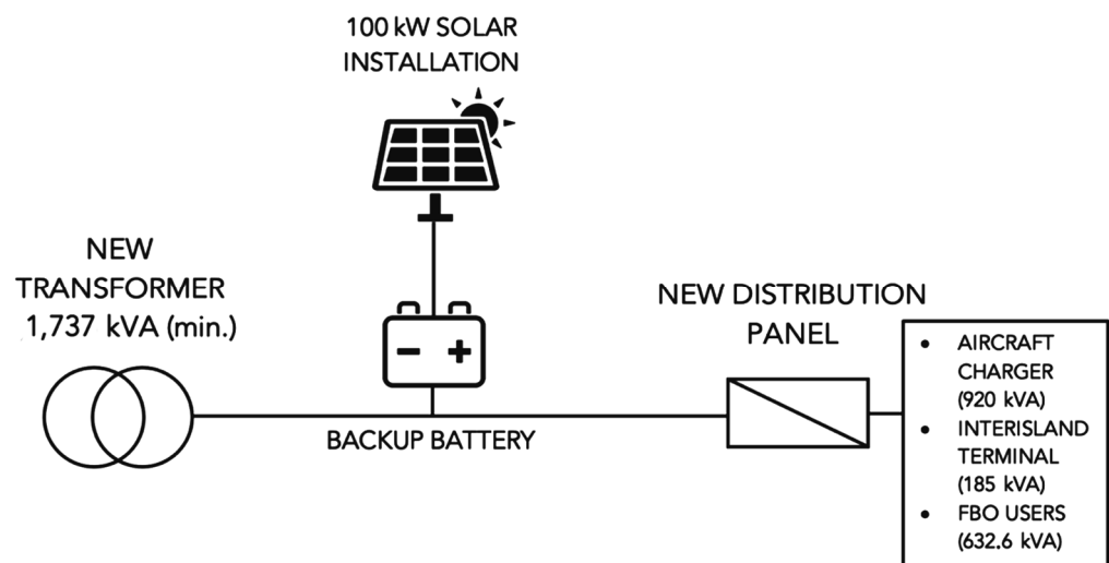
Figure 11. First concept drawing of a new electric infrastructure to install one charging station.
