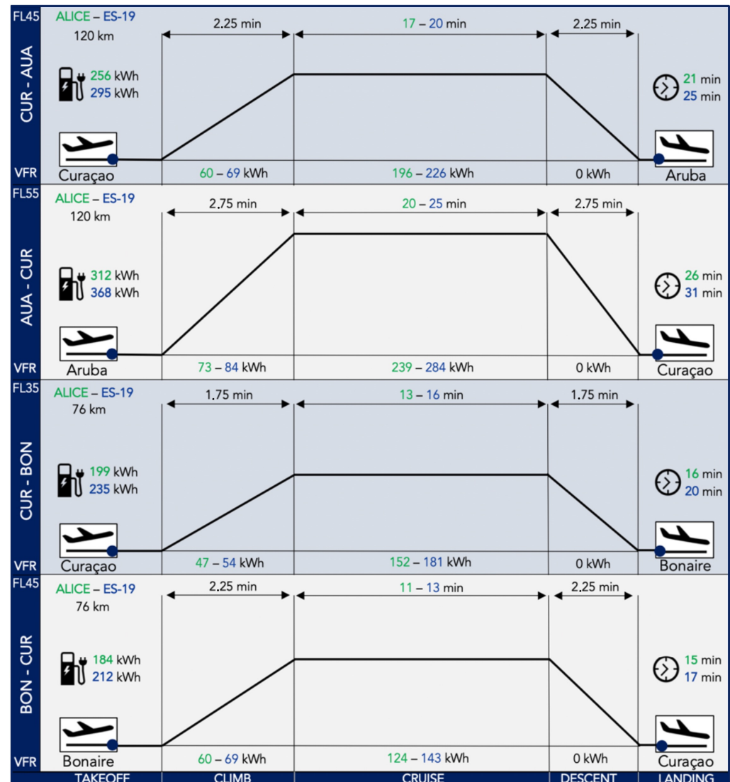
Figure 5. Interisland mission profiles for the four routes (green: Alice, blue: ES-19).
