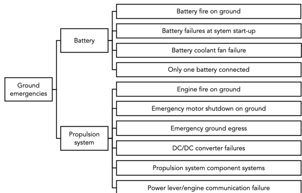
Figure 13. Ground emergencies that could occur with electric aircraft, based on the POH of the Pipistrel Velis Electro [31].
