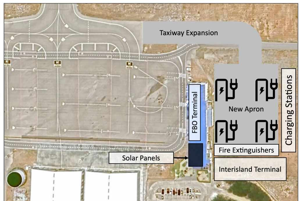
Figure 9. Second conceptual design of the new terminal at the south side of Aruba Airport.
