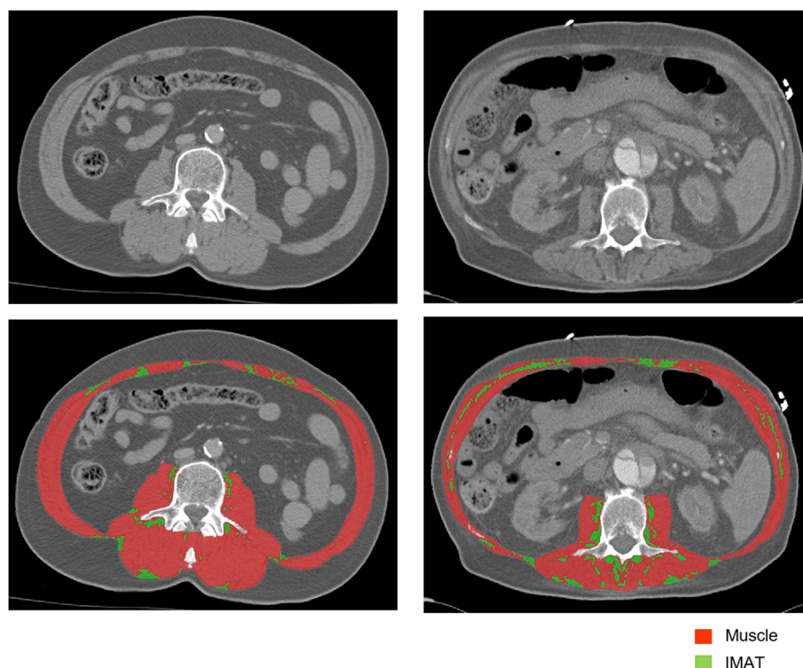
Fig. 1 Example of CT scan analysis. This image shows CT scans at the level of lumbar vertebra 3 of two patients both un-analysed (upper row) and analysed (lower row). The analysed images show muscle tissue (red) and intermuscular adipose tissue (IMAT, green). The patient on the left has more muscle ( 165 vs. 120 \text{ cm}^2 ), less IMAT ( 10 vs. 19.5 \text{ cm}^2 ), and higher mean skeletal muscle density ( 42 vs. 18 Hounsfield Units) than the patient on the right
