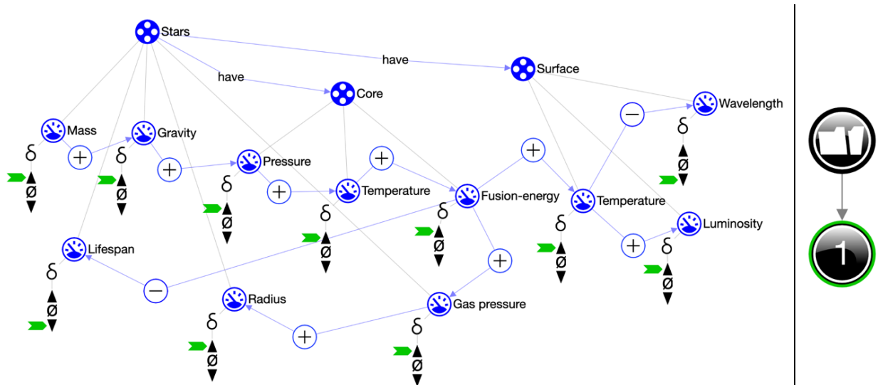
Figure 3. Simulation result for the star properties model shown in Fig. 2. Each quantity has a \delta which can be decreasing (arrow down), steady ( \emptyset ), or increasing (arrow up). Starting with Mass increasing, the simulation shows how other quantities change depending on their proportional relationship with the preceding quantity.
