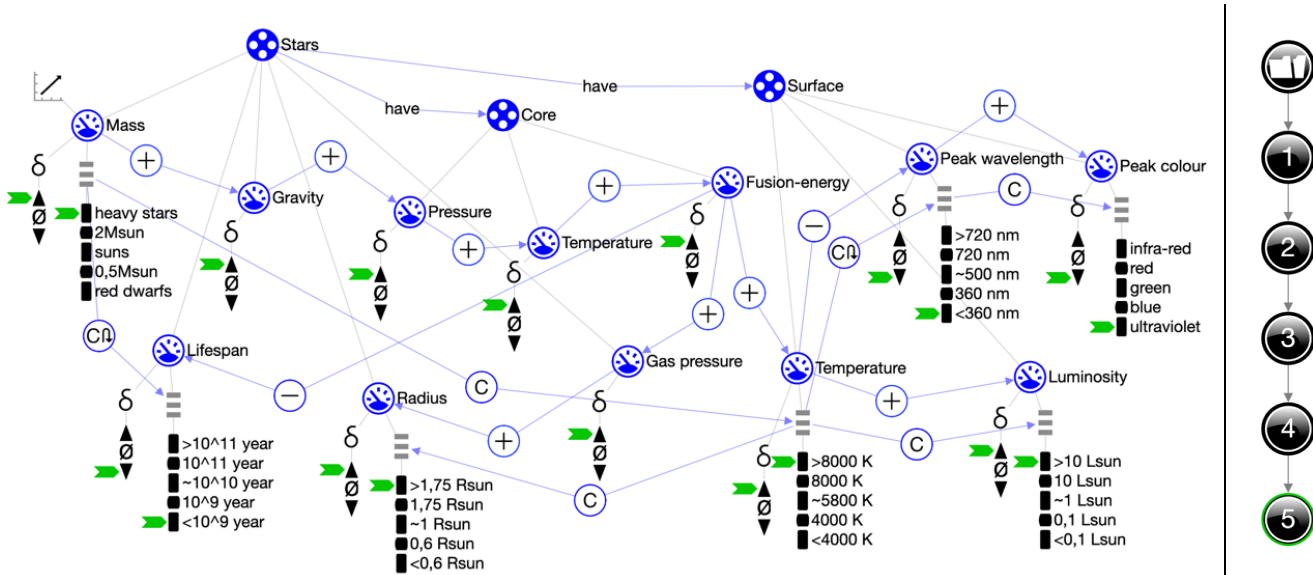
Figure 4. Part of the simulation results for the star states model. The simulation started with Mass =<red dwarfs, +> (not shown). Following this setting the six key quantities get their initial value via correspondences (C), notably, Lifespan started at < 10^9 year, Radius at <0.6 Rsun , Temperature at <4000 K, Luminosity at <0.1 Lsun , Peak wavelength at <360 nm, and Peak colour at infra-red. The derivatives are calculated using the causal dependencies (-, +). The state-graph (RHS) shows that the simulation progressed through 5 states. State 5 is shown (LHS).
