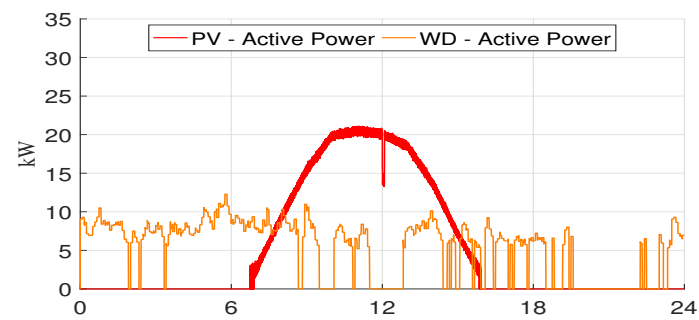
(b) PV and wind production
