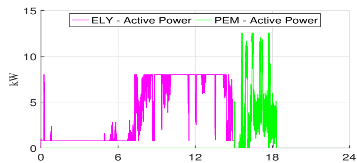
(c) ELY consumption and PEM production
