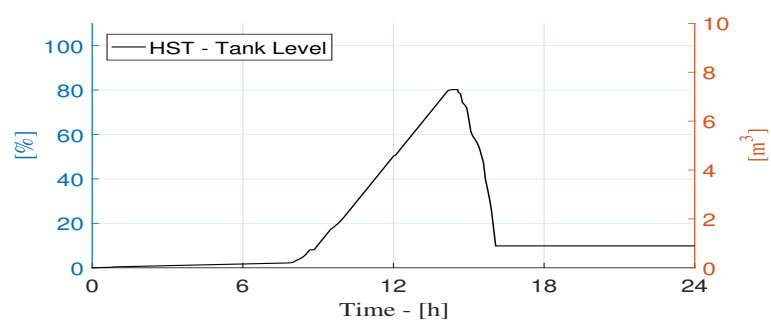
(e) Tank level
