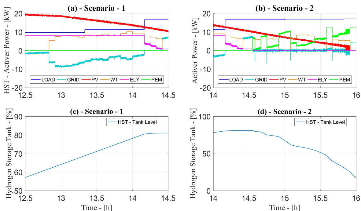
Figure 13. Global model performance of the H\mu G in different scenarios using a validation load profile. Scenario 1: H_2 production; both favorable wind and solar irradiance conditions. Scenario 2: H_2 consumption; scarce wind speed and solar irradiance conditions.
