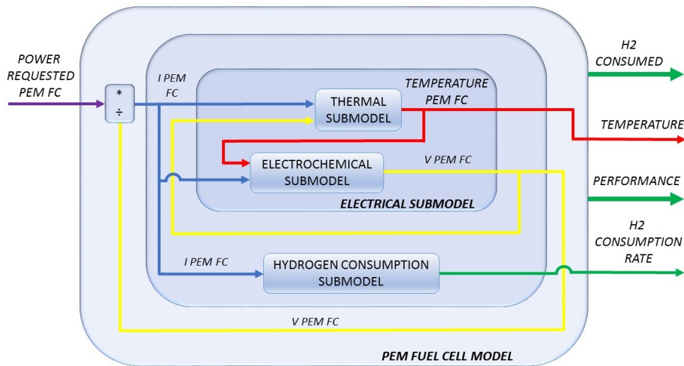
Figure 5. Block diagram of sub-models for a PEM fuel cell.
