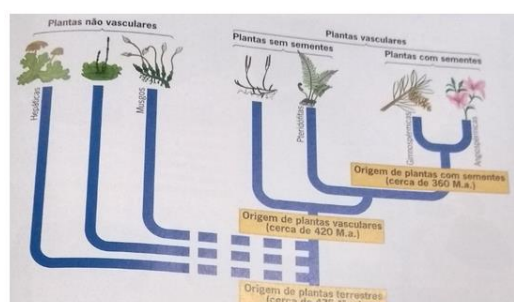
Figure 4. Phylogenetic cladogram
