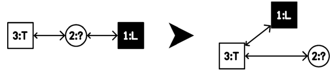
Fig. 9. Rule to move a lock forward. The circular node marked with a question mark indicates any node. Applying this rule will not change the type of this node, only its location and connections in the graph.
