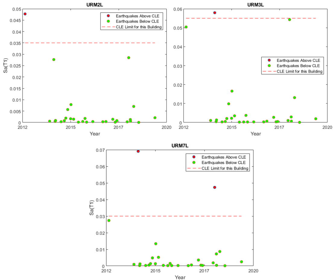
Figure 5. Elastic spectral acceleration demands for all earthquakes above magnitude M_L2.0 and comparison with the CLE spectral acceleration limits for building typologies URM2L (top-left), URM3L (top-right) and URM7L (bottom) - please note that the red dots show the earthquakes that would exceed the CLE level earthquake limit in the last y years, since 2012 Huizinge event.
